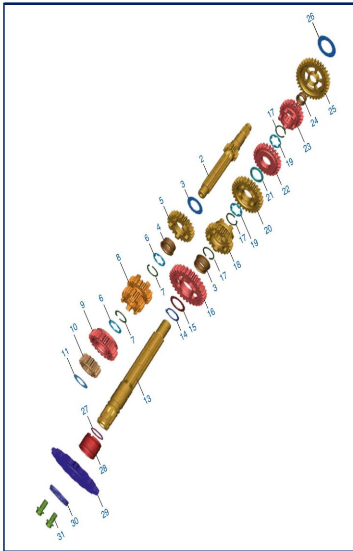
FIGURA N°7: TRANSMISION
